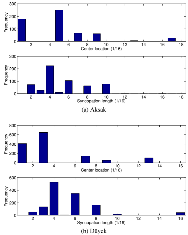
Figure 6: Syncopation localizations and lengths for usul Aksak and Düyek
