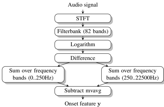
Figure 1: Computing the onset feature y from the audio signal
